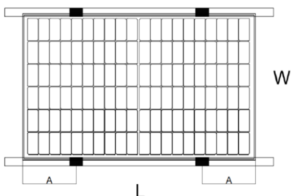
图 C 四点长边安装 导轨平行长边 Four point long side installation Guide rails are flush with long edges
