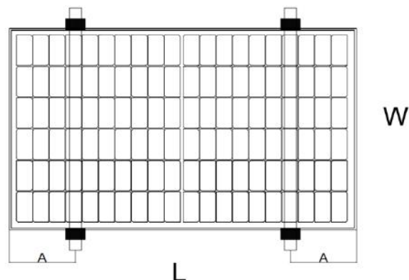
图 D 四点长边安装 导轨垂直长边 Four point long side installation Guide rail vertical long side
