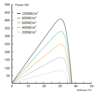
Power-Voltage Curve(410W)
